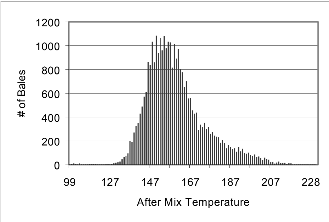
Figure 7 – After Mix Point Temperature Distribution
