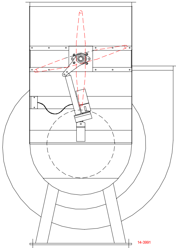
Figure 5 – Banjo Design View
