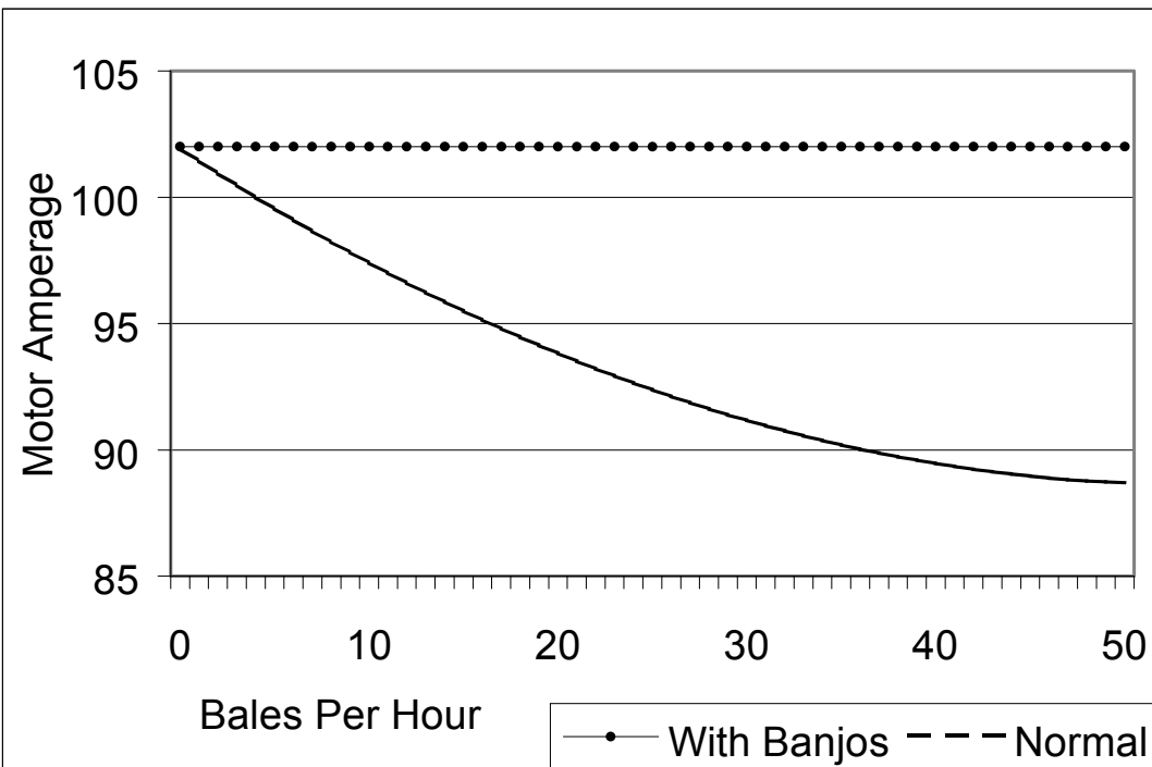
Figure 6 – Effect of Banjos on Motor Amperage as Bales Per Hour Increase
