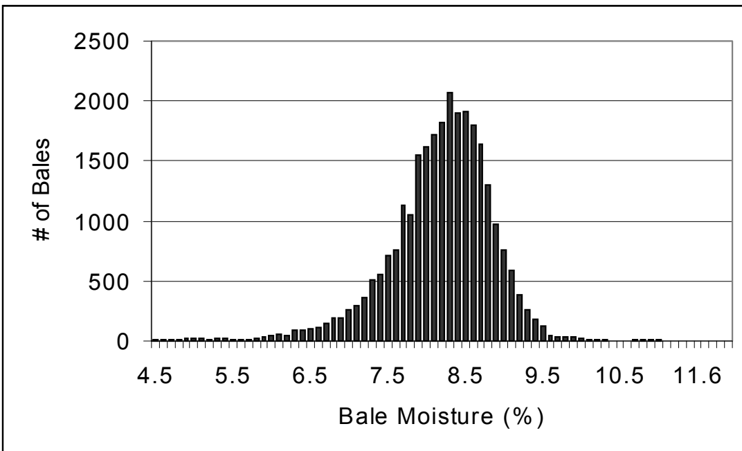
Figure 2 – Bale Moisture Distribution for Steamroller System
